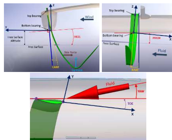
Figure 4: Appendage coordinate system
