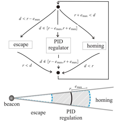
Fig. 6. Regulation diagram
