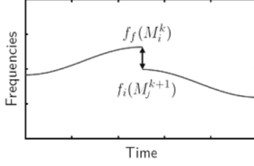
Fig. 6. C^0 time-frequency continuity.
